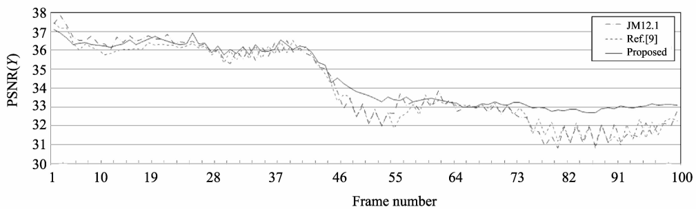
Fig. 1 Performance comparison of the proposed scheme with the PSNR value per frame (Table sequence, @30 Hz, 128 bps)
